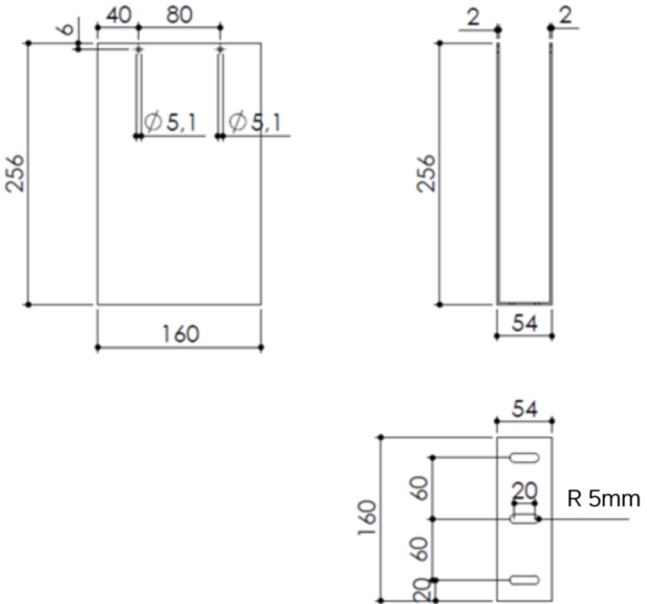
Figure A2a – Etrier (Tableau A2)
